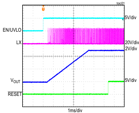
STARTUP THROUGH ENABLE ( V_{IN} = 24V , FIXED V_{OUT} = 5V , FULL LOAD, PWM MODE)
