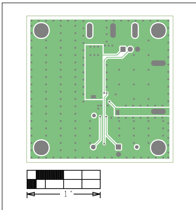
MAXM15464 EV Kit PCB Layout—Layer 3 Power
