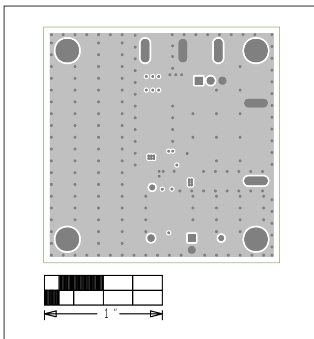
MAXM15464 EV Kit PCB Layout—Layer 2 Ground
