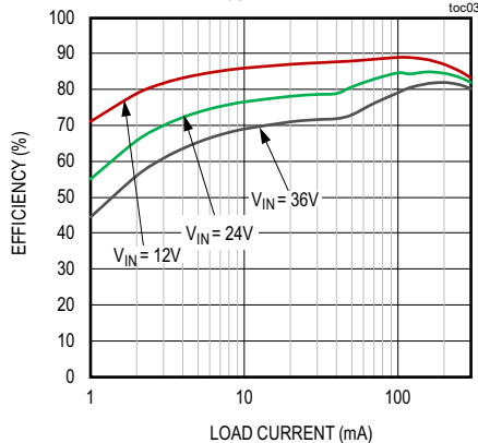
EFFICIENCY vs. LOAD CURRENT (FIXED V_{OUT} = 5V , PFM MODE)
