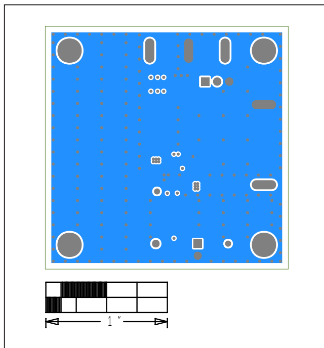
MAXM15464 EV Kit PCB Layout—Bottom Layer
