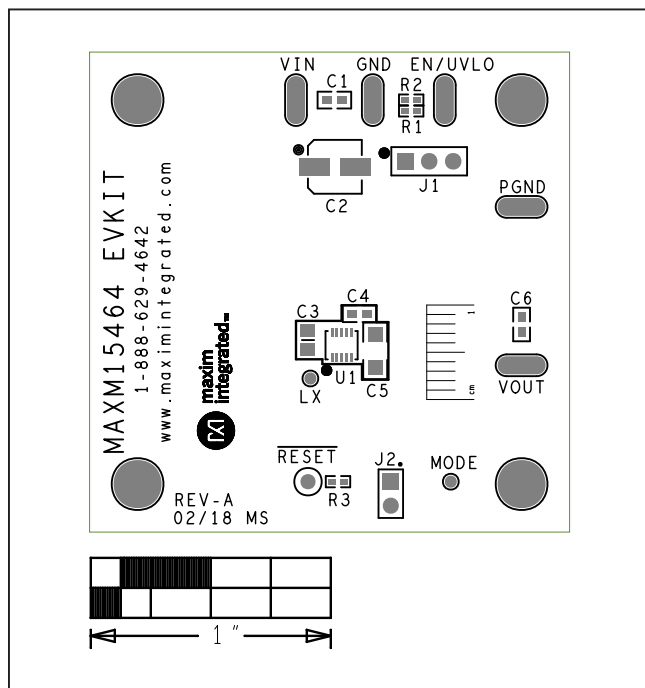
MAXM15464 EV Kit PCB Layout—Silk Top
