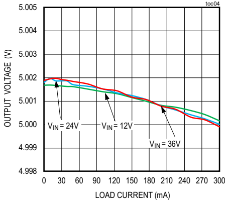
OUTPUT VOLTAGE vs. LOAD CURRENT (FIXED V_{OUT} = 5V , PWM MODE)
