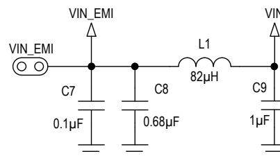
Figure 1. EMI Filter Components
