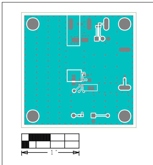
MAXM15464 EV Kit PCB Layout—Top Layer
